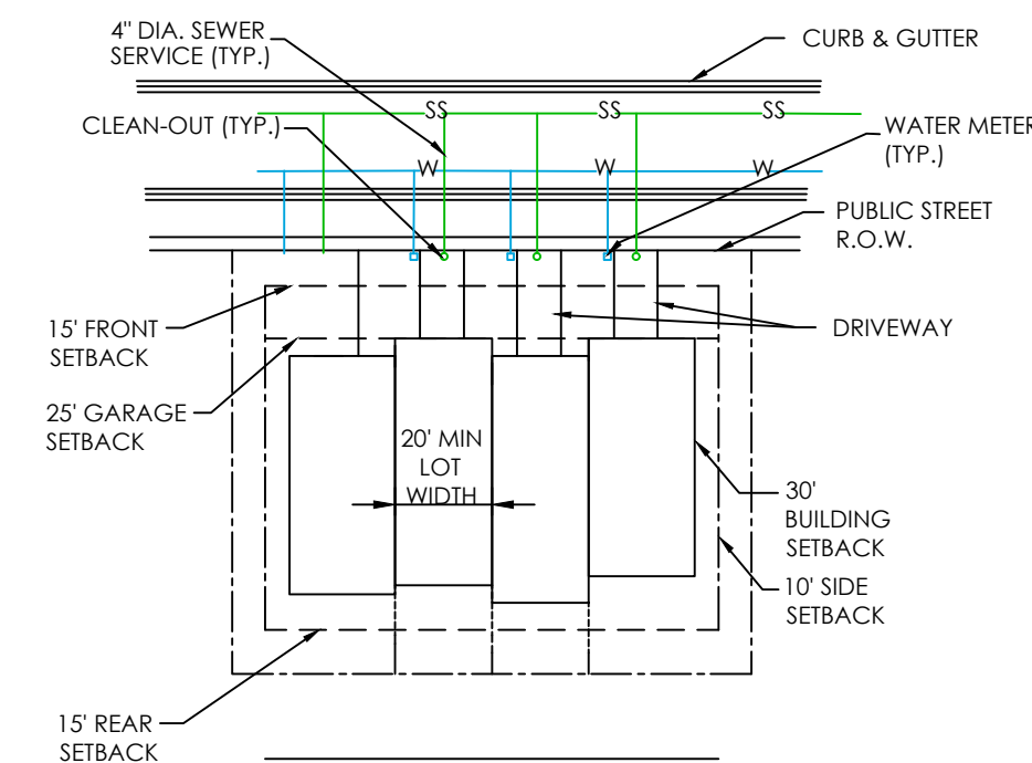
TYP LOT DETAIL - TOWNHOMES
