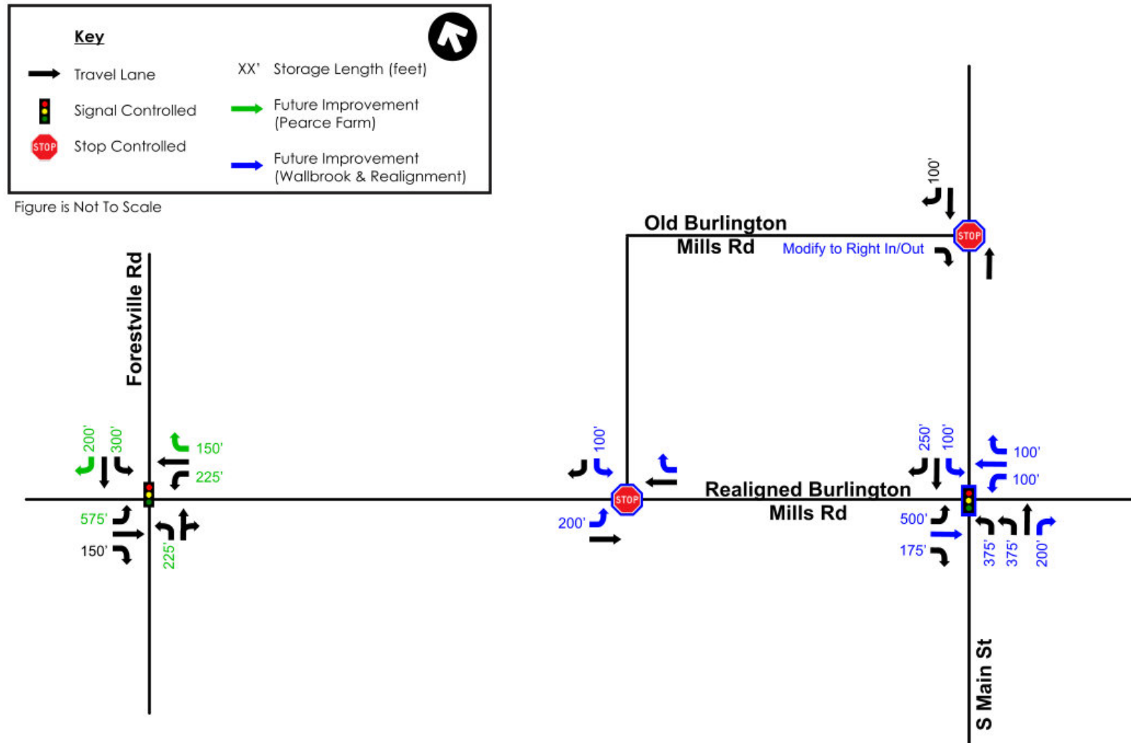
Figure 4: 2030 No-Build Lanes and Traffic Control
