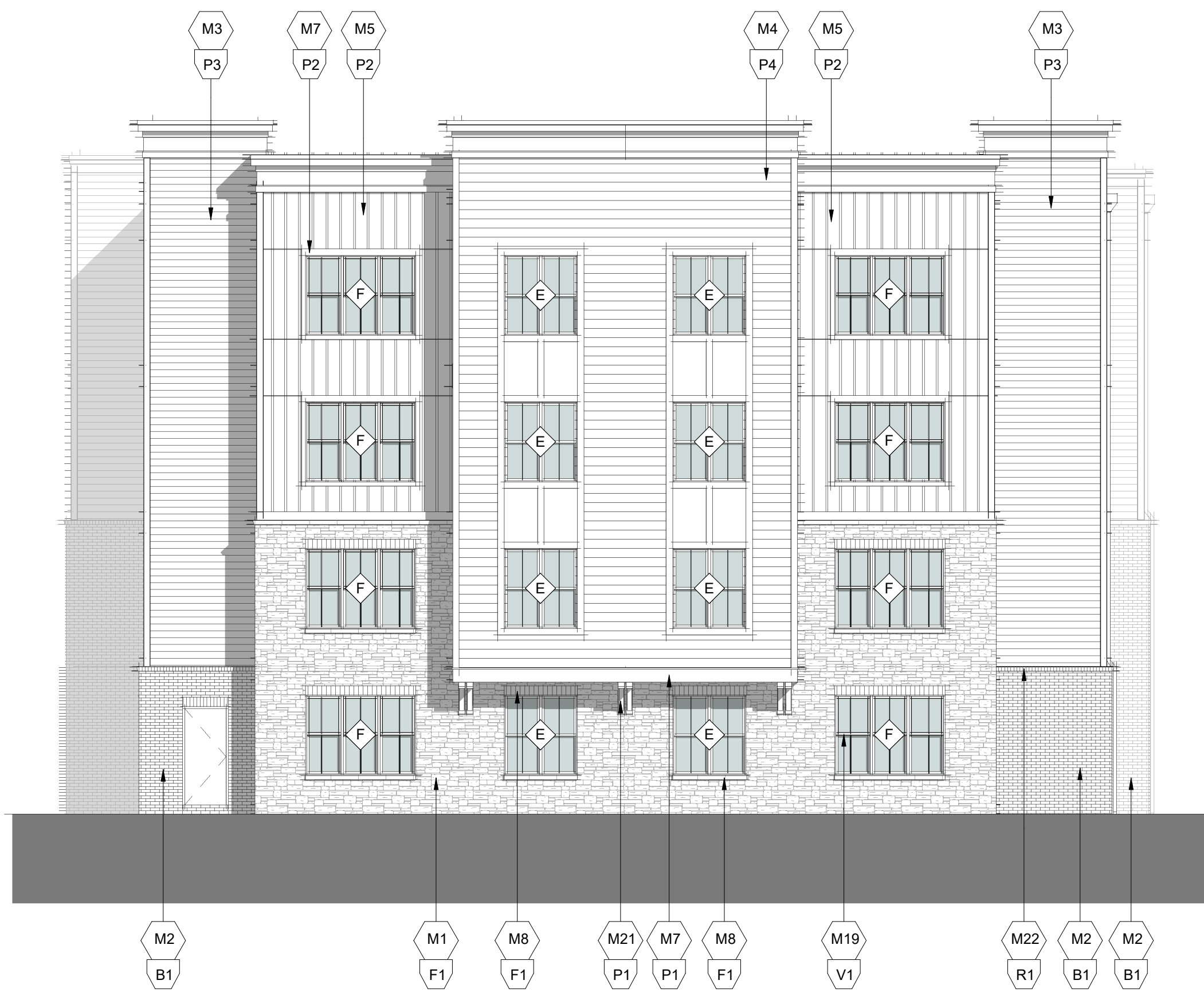
BLDG TYPE 2 - RIGHT SIDE ELEVATION 4 1/8" = 1'-0"
