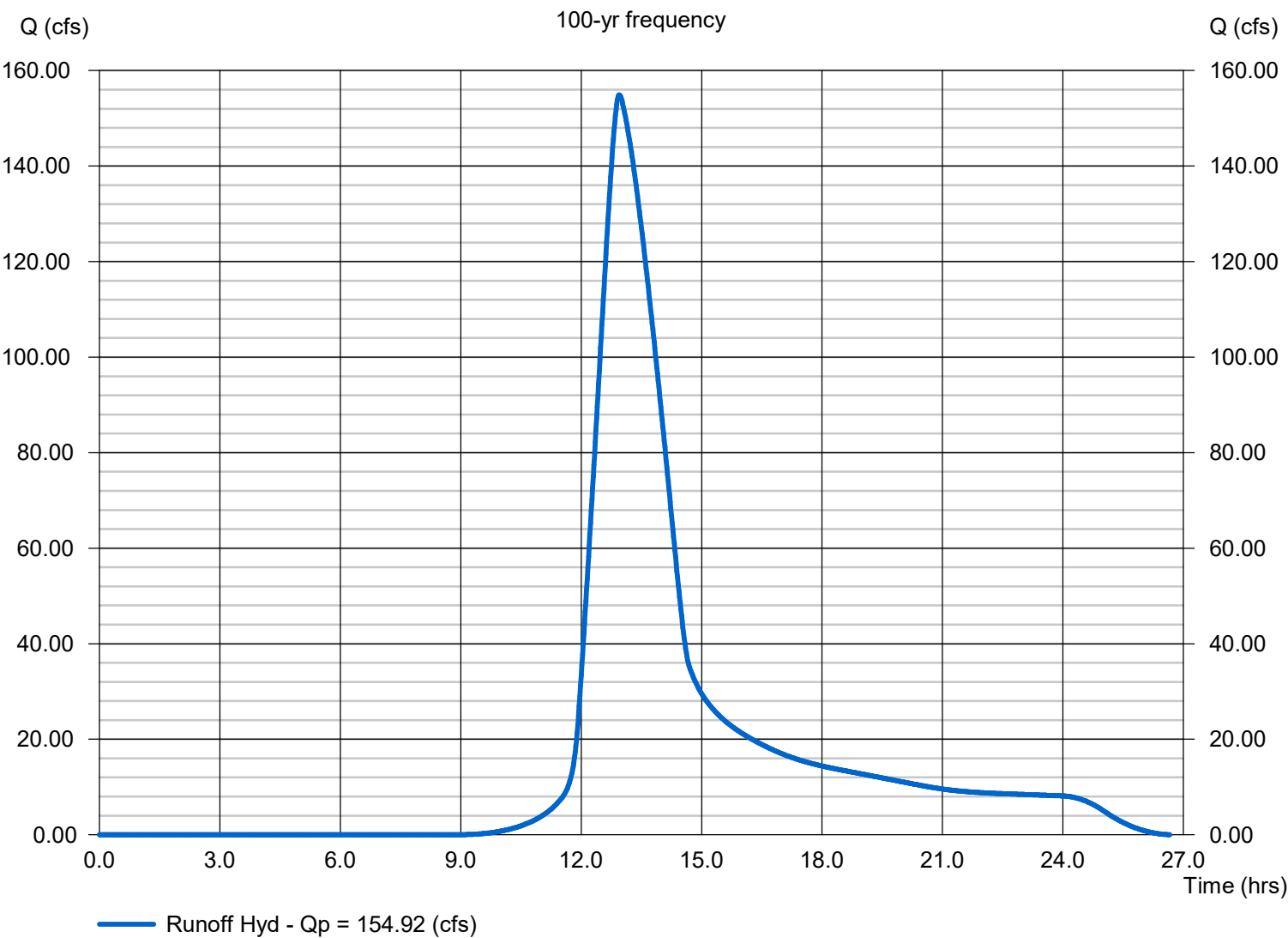
Runoff Hydrograph
