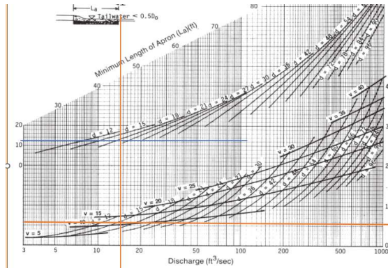
Figure 8.06a Design of outlet protection protection from a round pipe flowing full, minimum tailwater condition ( T_w < 0.5 diameter).
