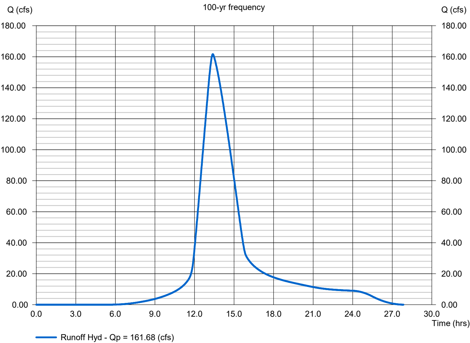
Runoff Hydrograph
